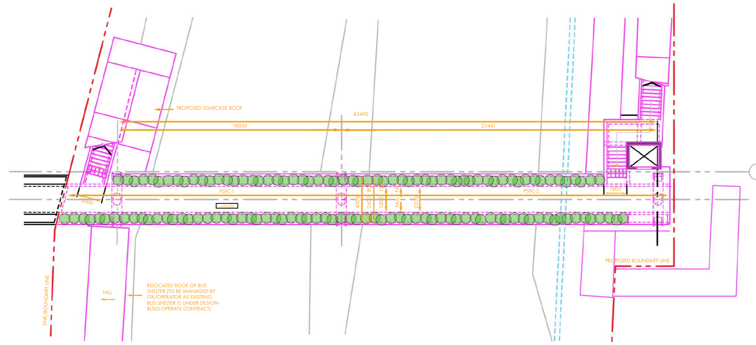
Sample Plan J: Showing the Planting Scheme along the Planter Troughs
